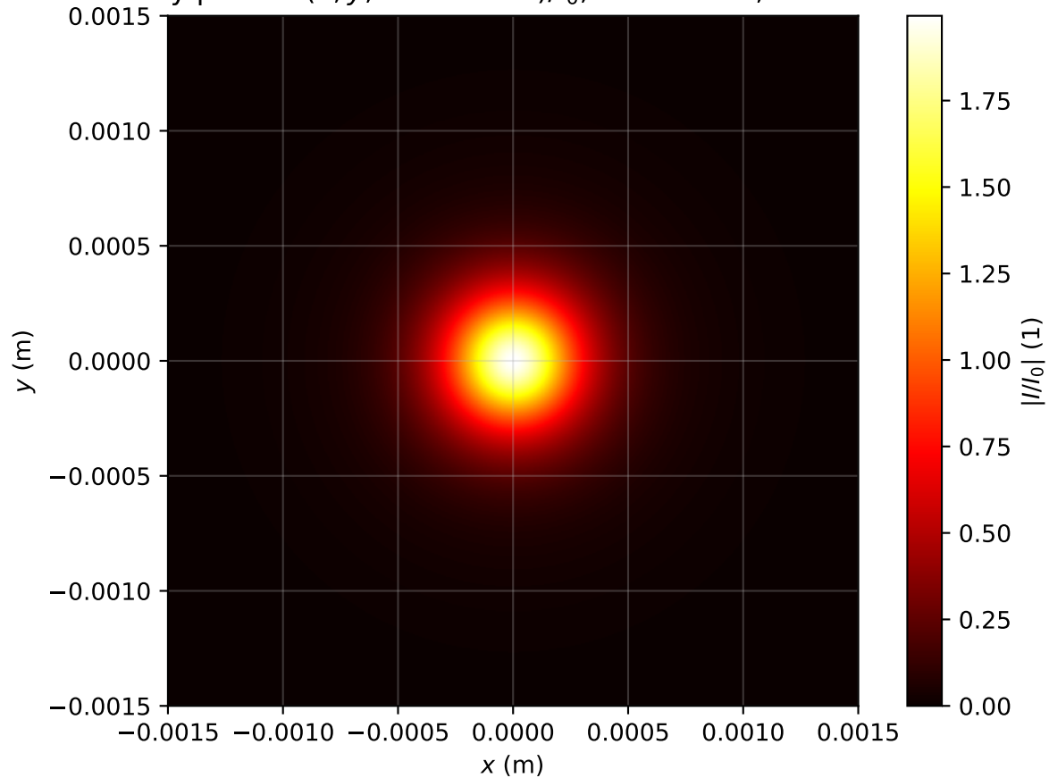
Intensity profile I(x, y, z = 1.751m)/I_0 , P_{in}=1.0P_{cr} , artificial time
